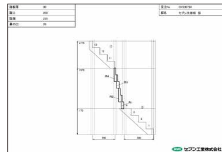
[内回り部材立面図]
