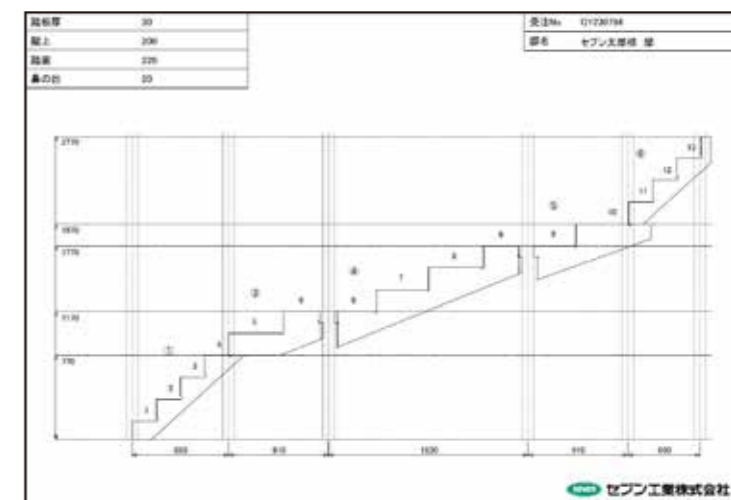
[外回り部材立面図]
